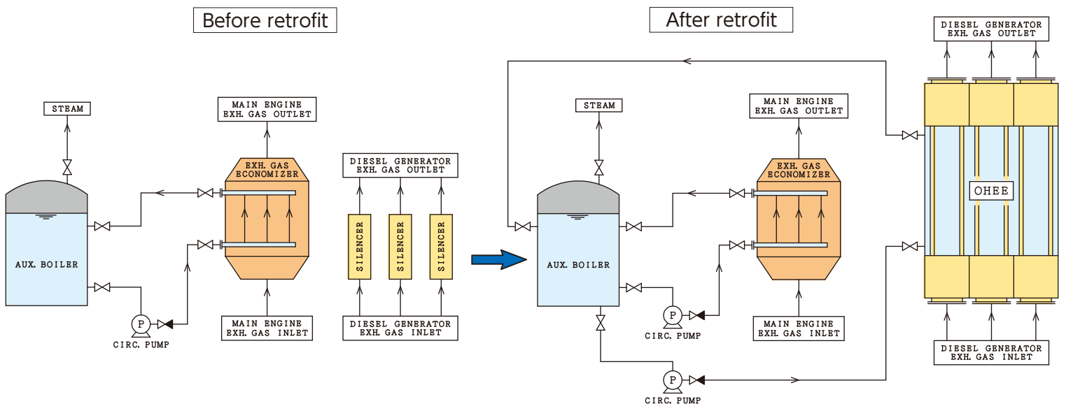
系統図 DIAGRAM FOR RETRO-FITTING
